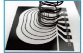
Measure gauge to determine the size of wire correctly
